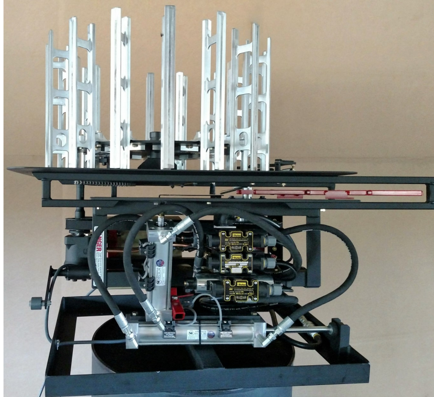
Fully Automatic Pat-Trap® Wobble Singles/Doubles Trap Machine
