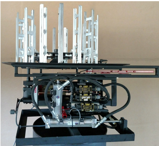
Standard Pat-Trap with Four Case Turret
